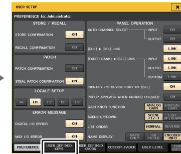
USER SETUP 窗口
